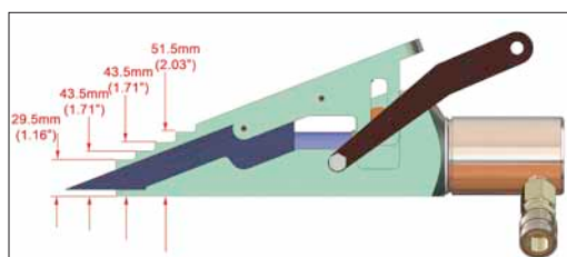
Wedge, opened
