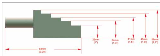
Safety block
