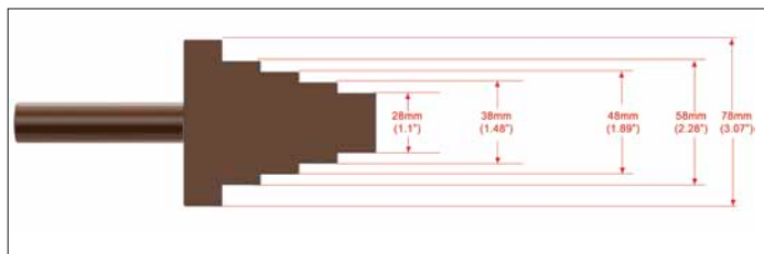
Safety block, side view
