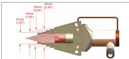
Wedge, opened
