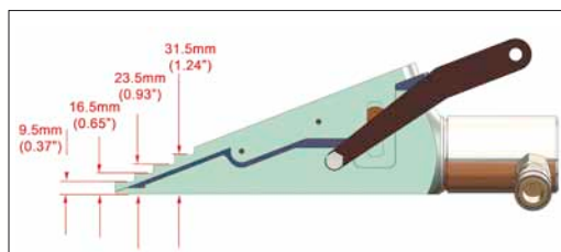
Wedge, closed
