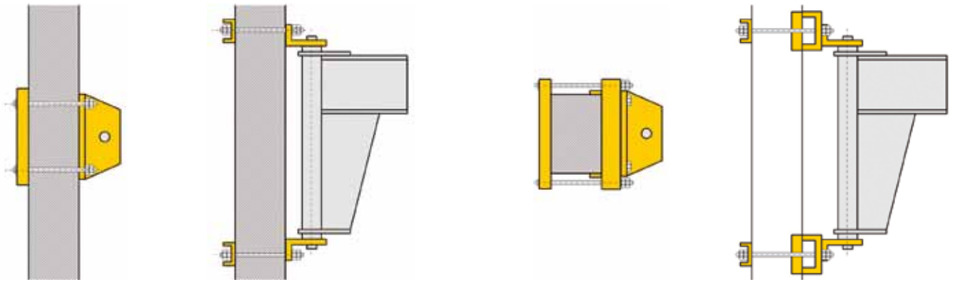
Wall mounting, using threaded rods going through the wall and being fixed to the wall with counter plates and nuts.
