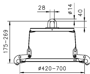
Model TFA-R
